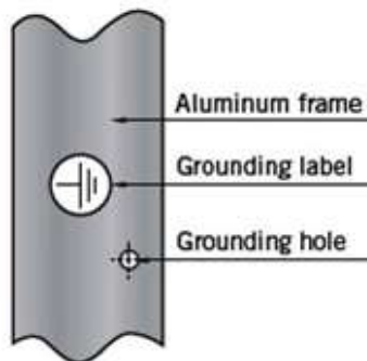
FIG 8-a Grounding hole
